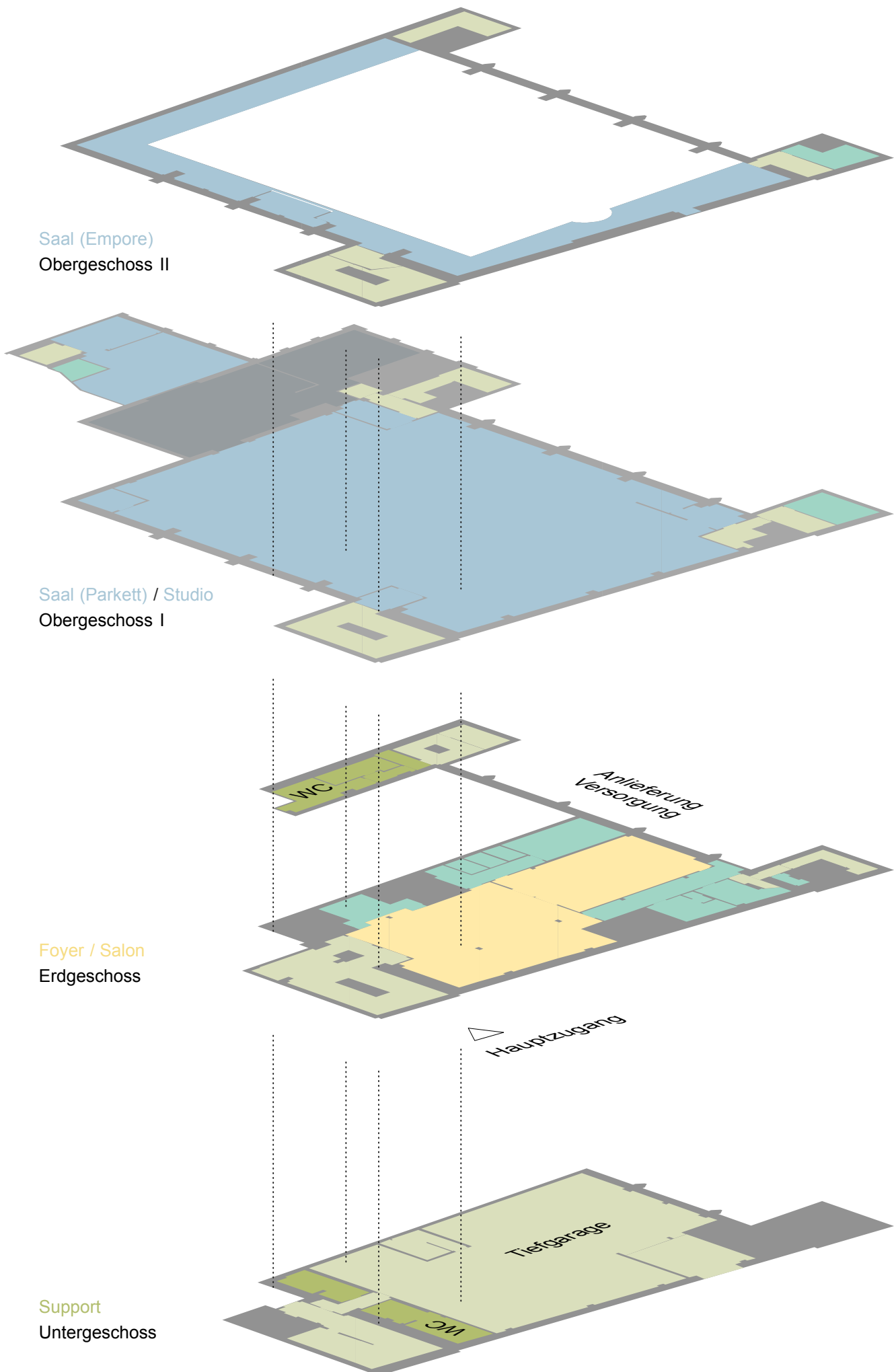
Isometrie Westbad Leipzig
